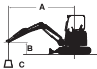
ZX55U-5A Cab Version, Blade above Ground Rating over-front Rating over-side or 360 degrees Unit: 1 000 kg
